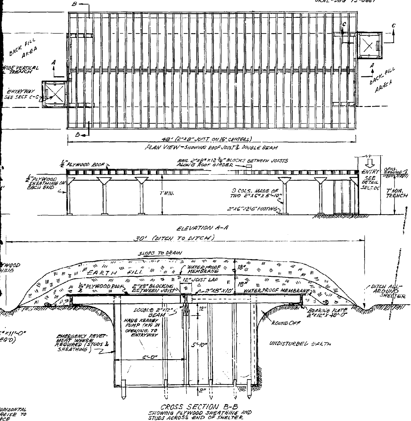
Fig. A-8.1. Trench Walls, Underground Shelter.
